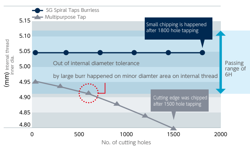
No. of cutting holes and internal thread inner dia
