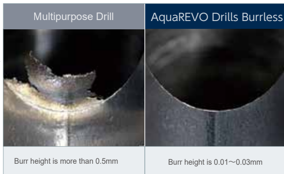
Burr height (Same diameter cross hole)
