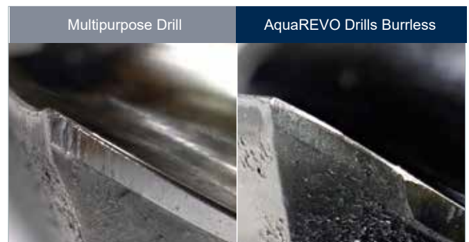
Tool wear after 120m cutting length
